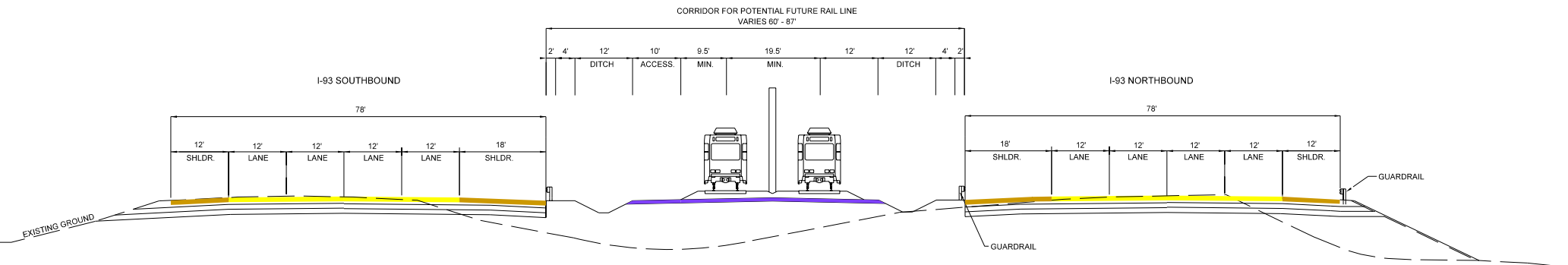
FOUR LANE TYPICAL SECTION OF IMPROVEMENT
