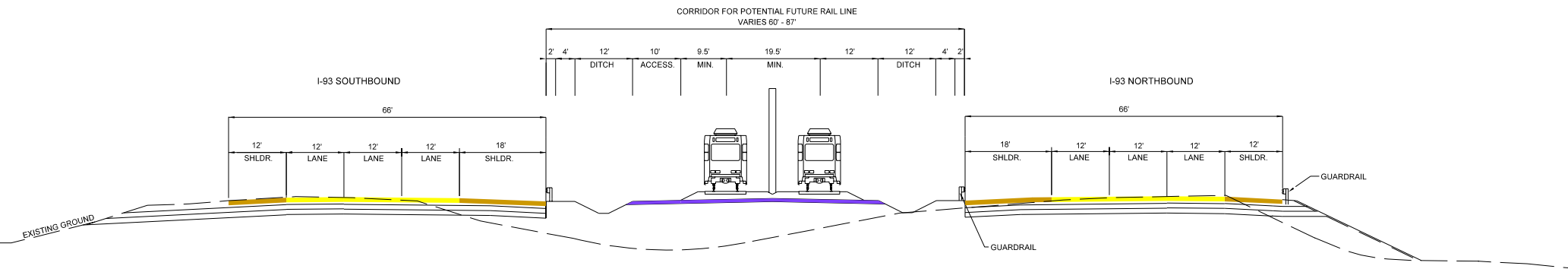
THREE LANE TYPICAL SECTION OF IMPROVEMENT
