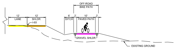
BIKE PATH TYPICAL SECTION
